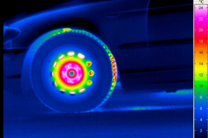
Test ABS
